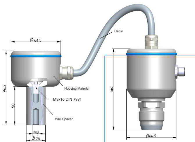
Example Sensor for mounting the DES e. g. SLI03, SDT03, STS...
